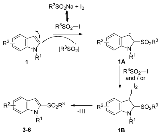
Scheme 1. Proposed Reaction Mechanism
