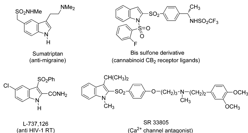
Figure 1. Representative examples of biologically active indolyl aryl sulfones.
